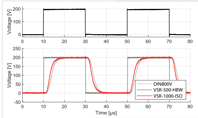
Fig. 3. Comparing VSR-1000-ISO with other imperix voltage sensors.
