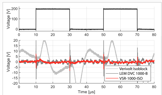
Fig. 6. Comparing VSR-1000-ISO with competing solutions.
