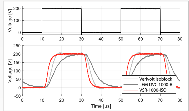
Fig. 4. Comparing VSR-1000-ISO with competing solutions.
