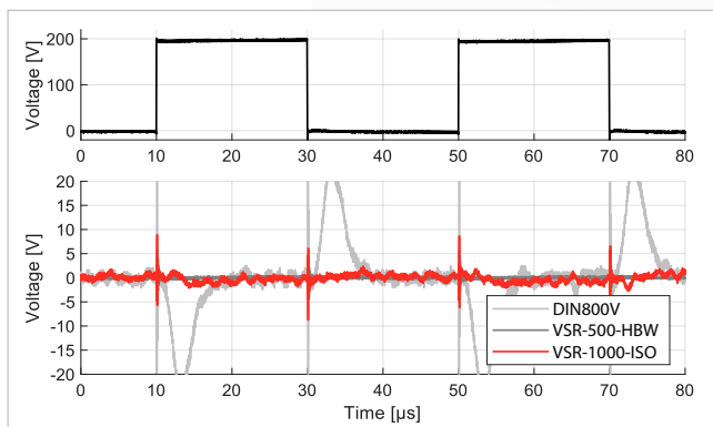
Fig. 5. Comparing VSR-1000-ISO with other imperix voltage sensors.
